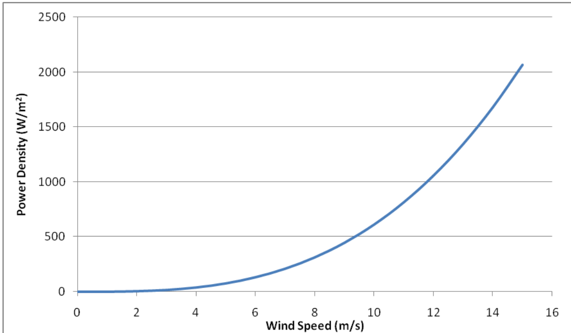
Figure 1. Power density versus windspeed – a cubic relationship.
