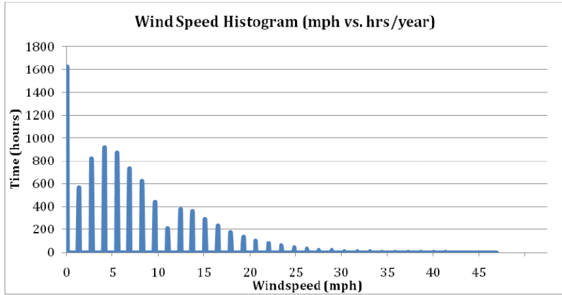
Figure 2. Silver Lake Rest Area wind speed histogram.
