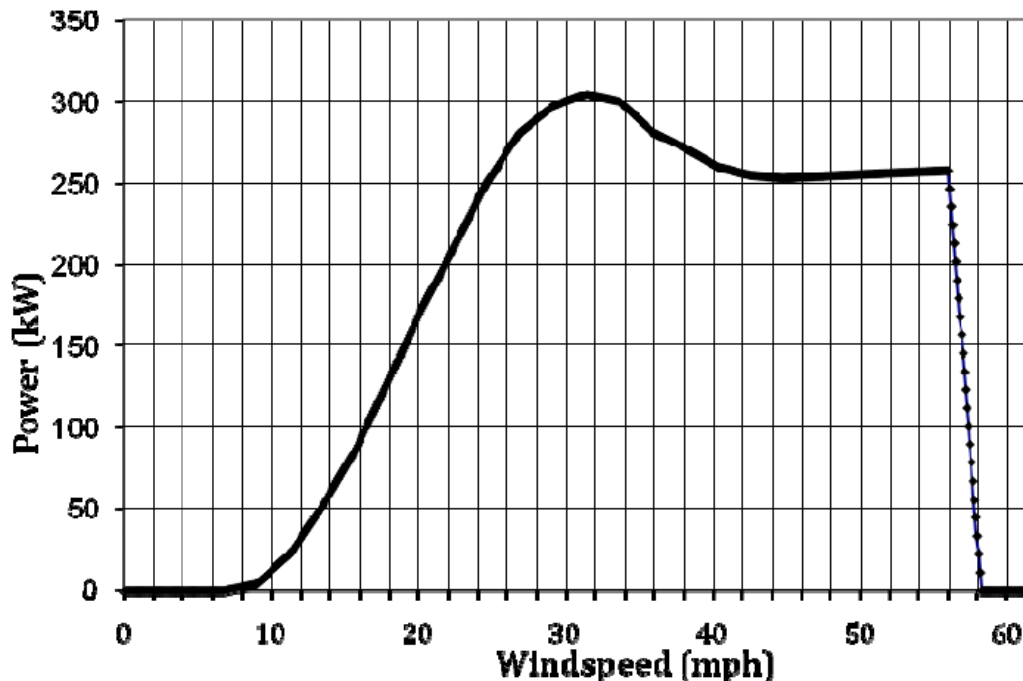
Figure 4. Power output versus velocity for the Bonus 300 kW Mk II (Idaho 2008)].
