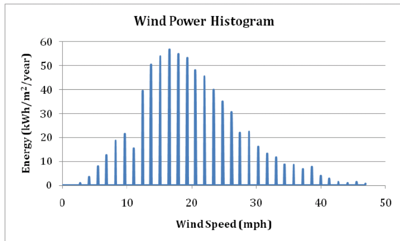
Figure 3. Average wind power, over one year, per square meter versus velocity for the Silver Lake Rest Area.
