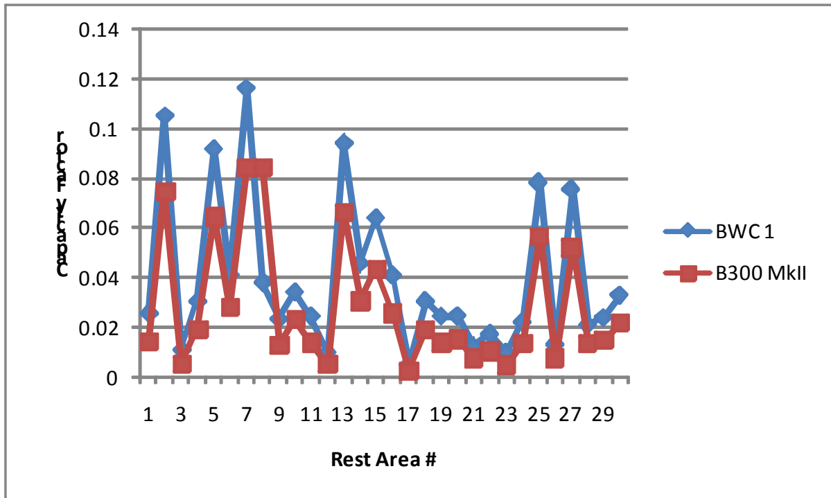
Figure 7. Comparison of capacity factor (CF) for the Bonus 300 kW Mk II and Bergey BWC 1 wind turbines for all rest areas (1-30).
