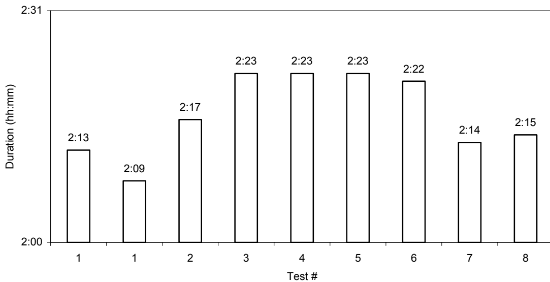
Figure 1. Duration of battery power (hh:mm) at full load for Myers UPS
