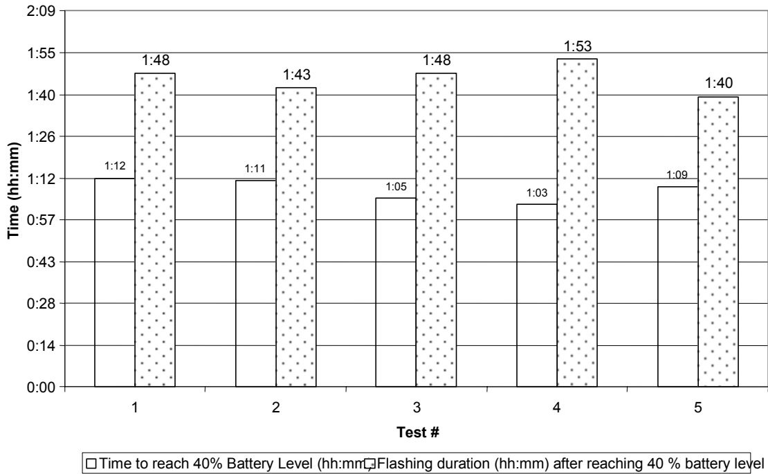
Figure 4. Myers UPS: Flash after reaching 40 % battery level
