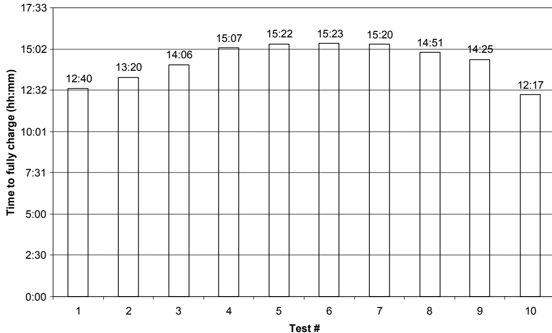
Figure 3. Time to fully charge the batteries (hh:mm) for Myers UPS
