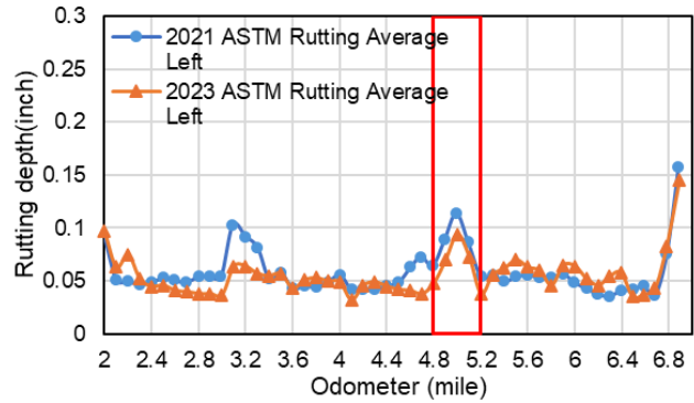
(b) Rutting average (left wheel path)
