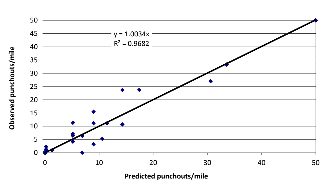
Figure 30. Graph. Accumulated damage versus observed punchout from current recalibration.
