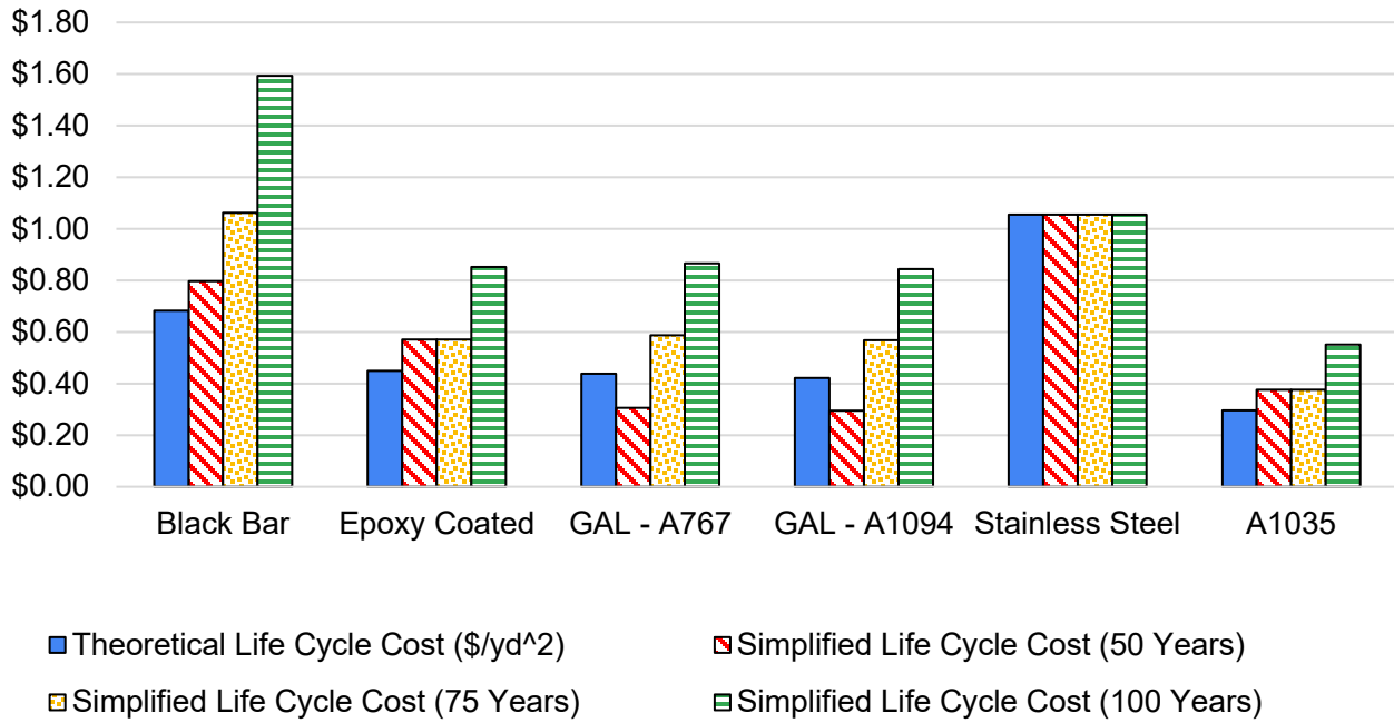
Figure 6. Graph. Graphical representation of life-cycle cost estimates for example 1.
