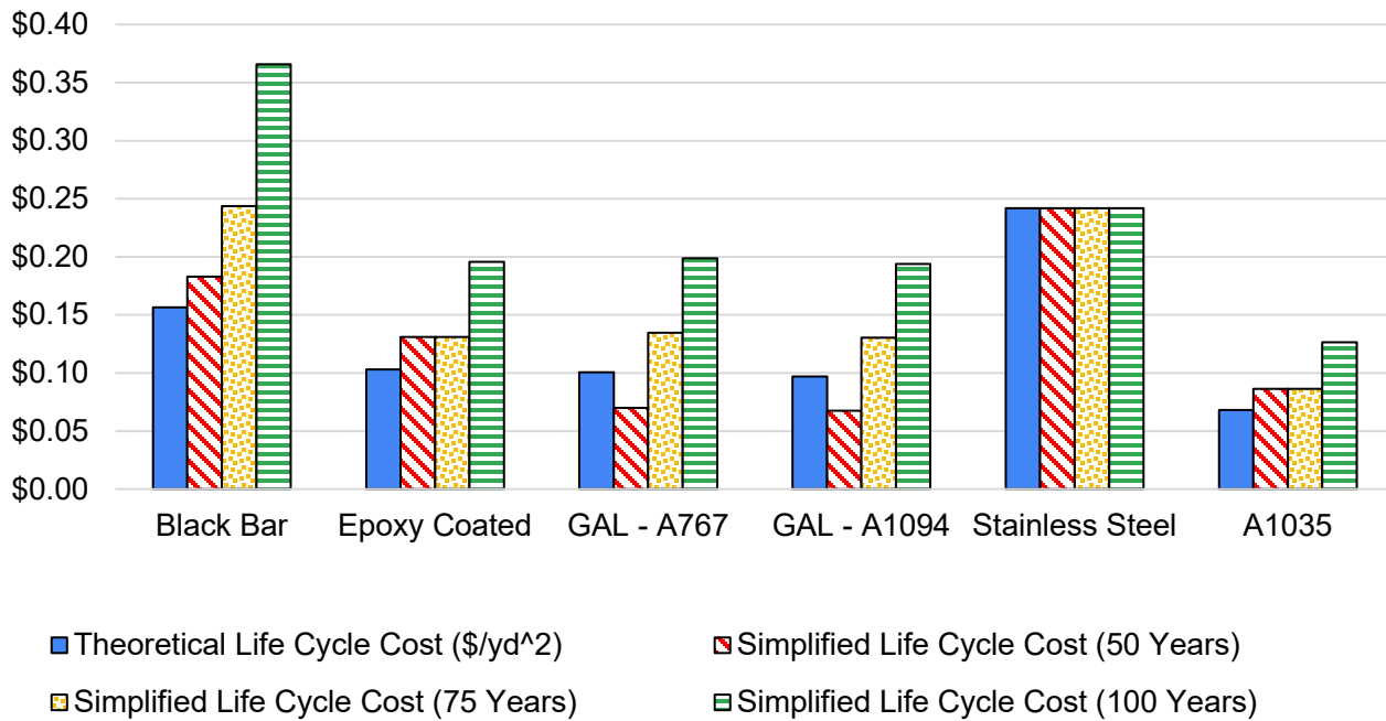
Figure 7. Graph. Graphical representation of life-cycle cost estimates for example 2.
